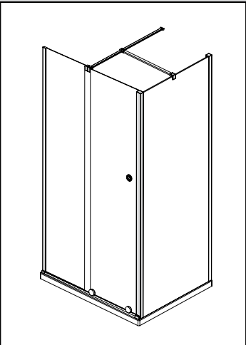
SLIDER & SIDE PANEL (Door closing against Side Panel) Rolla 8 door + Side Panel + Corner Post
