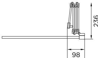
AQ9357LS/RS Swiftseal Semi Frameless 4 Fold Bath Screen Available as left or right hand option
