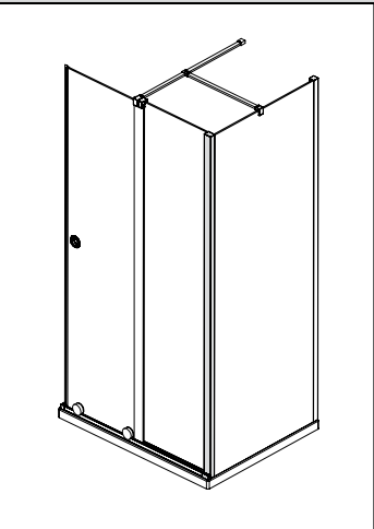
SLIDER & SIDE PANEL (Door closing against Wall/Window) Rolla 8 door + Side Panel + Corner Post + Closing Seal
