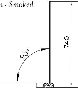
AQ6000-SM Square Edge Bath Screen - Smoked
