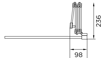
AQ9357LS/RS Swiftseal Semi Frameless 4 Fold Bath Screen Available as left or right hand option
