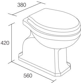
Low/High Level WC ceramic LA9116 £289 inlet height 360mm
