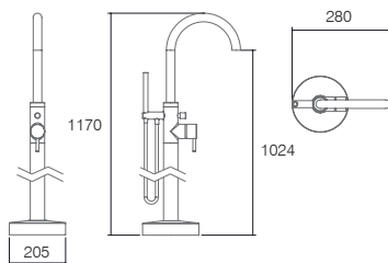
Freestanding Bath Shower Mixer* chrome LA1020 £540
