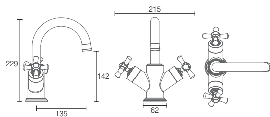
Basin Mixer with Click Waste chrome LA1009 £191.50
