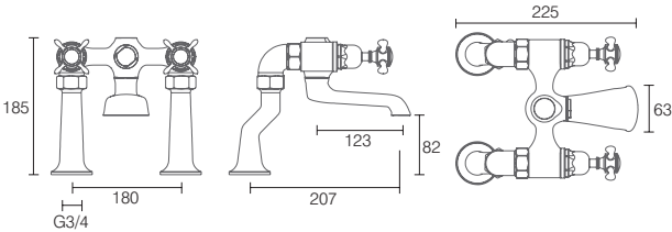
Bath Filler chrome LA1017 £225.50
