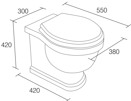
Back to Wall WC ceramic LA9127 £328
