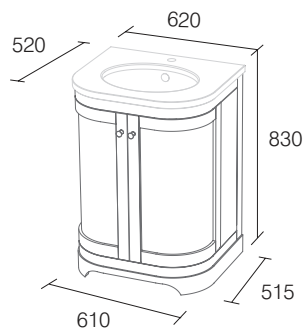
600mm Freestanding Basin Unit cotton white LA13061 £810 cobblestone LA13060 £810 charcoal LA13068 £810 (excludes worktop & basin)
