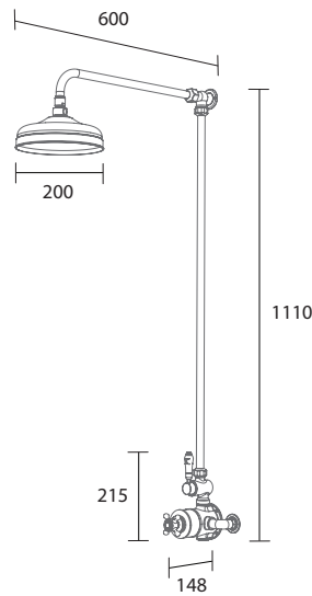
Clifton Exposed Single Function Shower System chrome LA3002 £595
