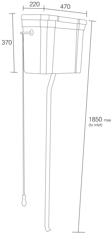
High Level Cistern 6L & Pipe/Fittings Kit ceramic cistern LA9118 £151.50 chrome pipe kit & cistern fittings LA9145 £434
