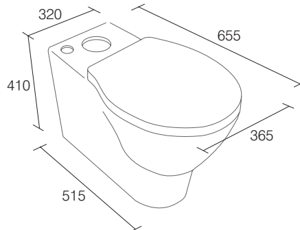
Close Coupled WC ceramic LA9106 £379
