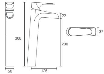
Tall Open Spout Basin Mixer with Click Waste* chrome LA1002 £191.50
