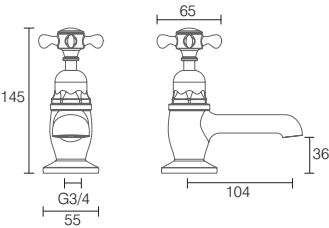
Bath Taps (pair) chrome LA1015 £112.50
