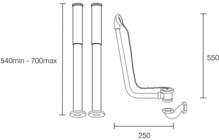
Exposed Chain Waste with Pipe Shrouds for use with deck mounted bath fillers & bath shower mixers min H540mm max H700mm 1½" waste chrome LA17002 £351
