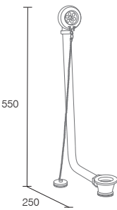
Exposed Chain Waste W250mm x H550mm 1½" waste chrome LA17001 £102.50
