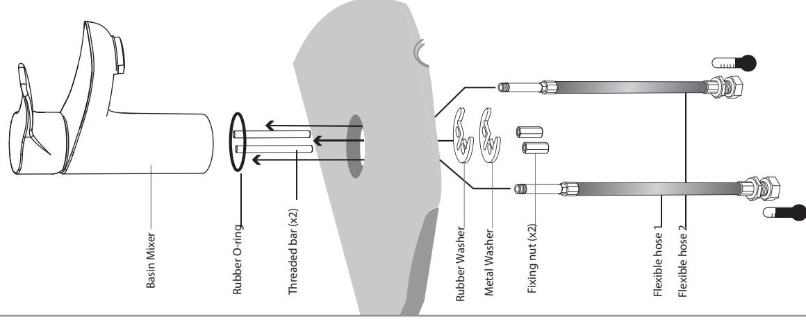
Basin Mixer Installation
