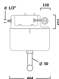
Apex dual flush slimline concealed cistern - side inlet
