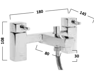
Bath Shower Mixer
