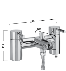
Bath Shower Mixer
