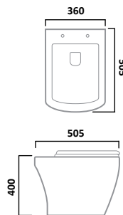
Back To Wall Pan
