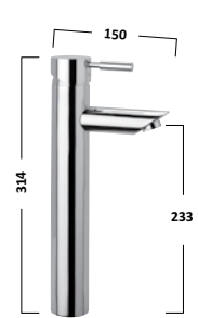
Tall Basin Mixer without Pop-Up Waste
