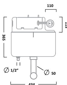
Vortex dual flush slimline concealed cistern - bottom inlet
