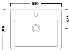
550mm Semi-Counter Top Basin 1 Tap Hole
