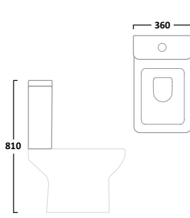
6/4L Cistern Inc Flush Fittings
