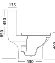
Close Coupled Pan Inc Floor Fittings
