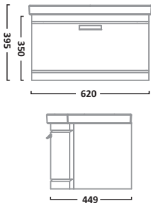
650mm Wall Mounted Unit
