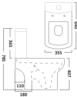
Open Back Close Coupled Pan & Soft Close Seat
