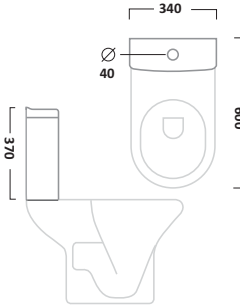
6/4L Cistern Inc Flush Fittings
