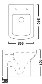
Back To Wall Pan With Soft Close Seat
