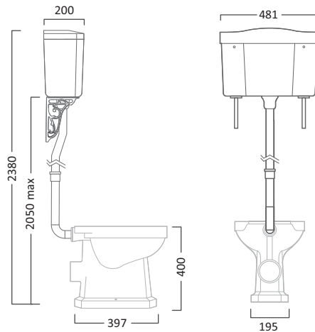
High level Ceramic Cistern Including fittings with Chrome Down pipe with Ornate Bracket & Flxing Kit
