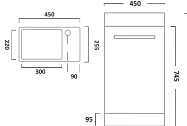
450mm Freestanding Unit & Ceramic Basin
