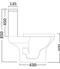
4.5/3L Cistern Inc Flush Fittings
