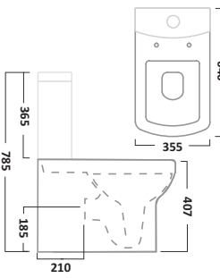
Flush Fitting Close Coupled WC Pan & Soft Close Seat
