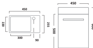
450mm Wall Mounted Unit & Ceramic Basin
