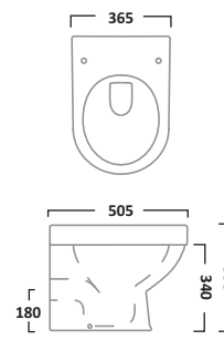
Back To Wall Pan
