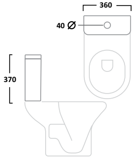
6/4L Cistern inc. Flush Fittings
