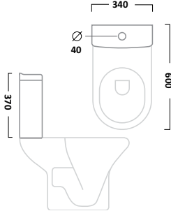
6/4L Cistern Inc Flush Fittings
