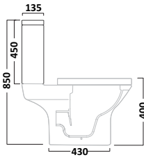
4.5/3L Cistern Inc Flush Fittings
