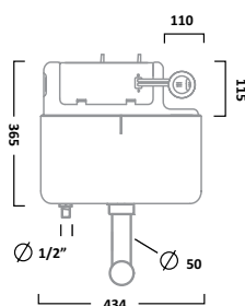
Vortex dual flush slimline concealed cistern - bottom inlet
