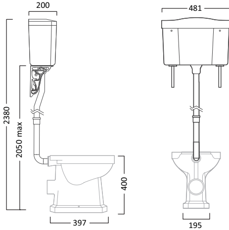
High level Ceramic Cistern Including Fittings with Chrome Down Pipe, With Overflow Bracket & Flange Kit
