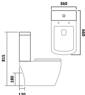
6/4L Cistern Inc Flush Fittings
