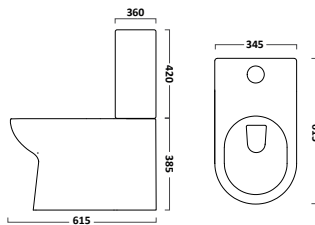
Fully Enclosed Close Coupled WC
