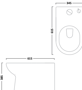
Fully Enclosed Close Coupled WC
