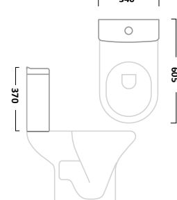
6/4L Cistern Inc Flush Fittings
