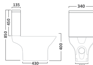
4.5/3L Cistern Inc Flush Fittings
