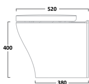
Back to Wall Pan Side View
