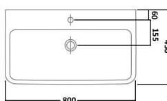
800mm Ceramic Basin 2 Tap Hole
