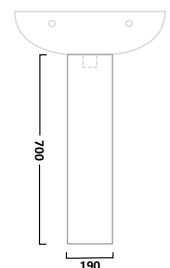
Full Pedestal (Suitable for 450 &amp; 565mm basins)
