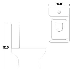
6/4L Cistern Inc Flush Fittings
