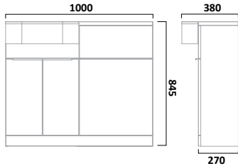
1000mm Semi-Countertop & Back To Wall Unit (Left)
