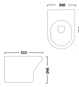
Wall Hung Pan
