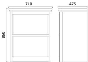
700mm Freestanding Unit
