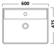
600mm Ceramic Basin
