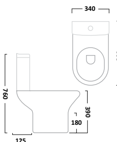
Short Projection WC Pan
