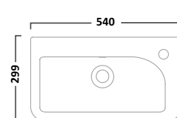
Semi-countertop Slim Depth Basin
