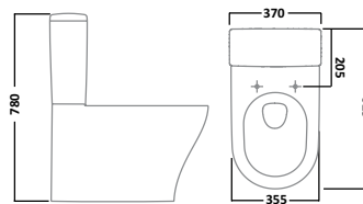
Close Coupled WC
