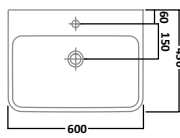
600mm Ceramic Basin 1 Tap Hole
