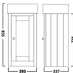
400mm Cloakroom Unit
