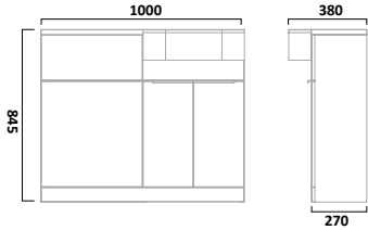
1000mm Semi-Countertop & Back To Wall Unit (Right)
