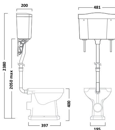
High Level Ceramic Cistern including Fittings with Chrome Down Pipe, Ornate Bracket & Flxing Kit
