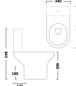
Comfort Height Pan
