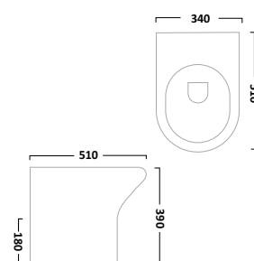
Short Projection Back To Wall WC Pan
