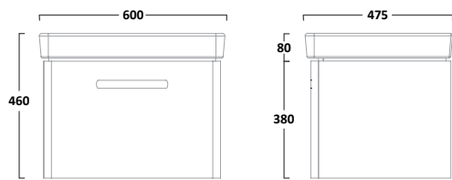
600mm Wall Mounted Unit
