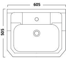
605mm Ceramic Basin - 1 Tap Hole
