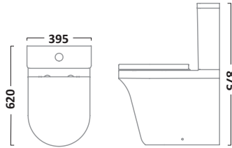
Comfort Height Fully Enclosed Close Coupled WC Pan PCF650S Cistern C650S
