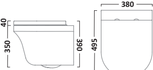
Comfort Height Wall Hung WC Pan WH650S
