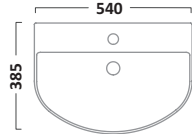
Slim Depth Semi-Countertop Basin 1 Tap Hole DC14005
