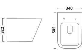
Wall Hung WC Pan WH450S
