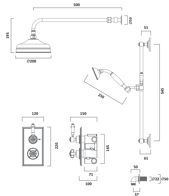
Thermostatic Concealed Dual Function Shower Valve with Shower Head & Handset Chrome
