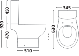
Comfort Height Fully Enclosed Close Coupled WC Pan PC450S Cistern C450S
