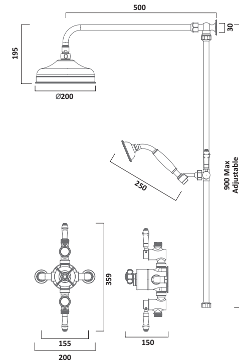
Thermostatic Exposed Dual Function Shower Valve with Shower Head & Handset Chrome
