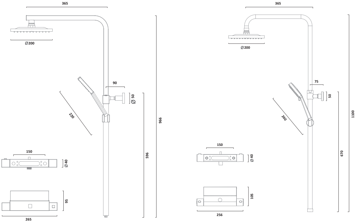
Dual Function Bar Valve with Shower Head & Handset Chrome SZN1508
