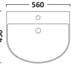
Semi-Countertop Basin 1 Tap Hole DC14004
