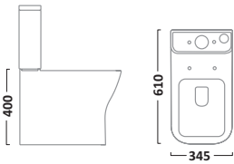
Fully Enclosed Close Coupled WC Pan PF450S Cistern C450S
