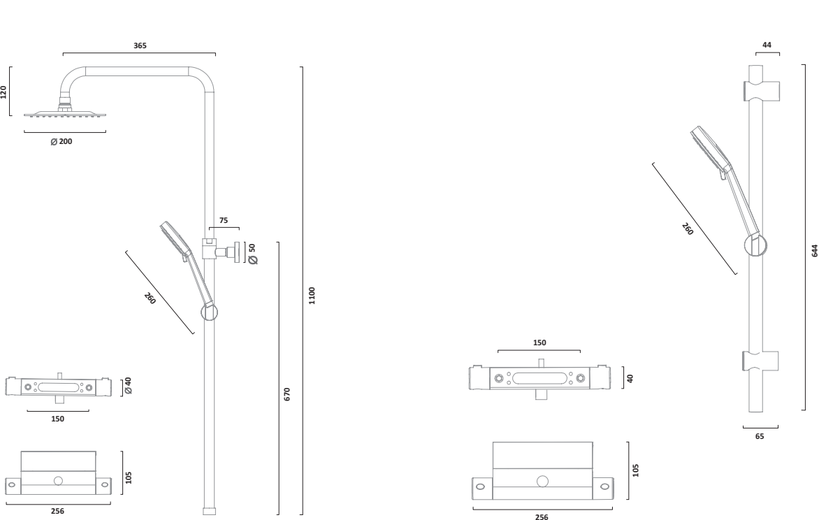
Cool Touch Thermostatic Dual Function Bar Valve with Shower Head & Handset Chrome SQT2209
