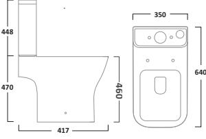
Comfort Height Open Back Close Coupled WC Pan PC455S Cistern C450S
