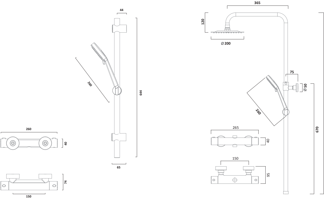
Cool Touch Thermostatic Single Function Bar Valve & Handset Chrome SQT2416
