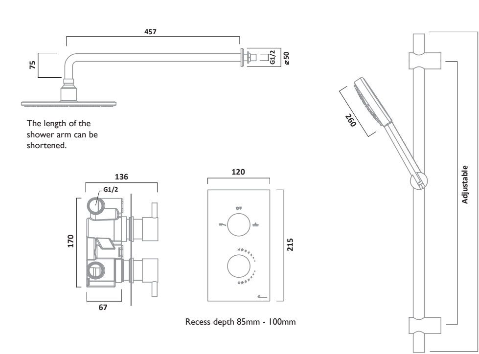
Thermostatic Concealed Dual Function Valve with Shower Head & Handset Chrome SQT1611
