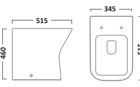
Comfort Height Back to Wall WC White BTWC450S
