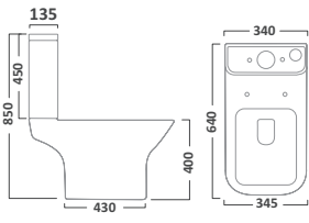
Open Back Close Coupled WC Pan P450S Cistern C450S
