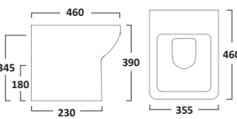
Back To Wall WC Pan BTW900S
