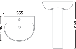
550mm Ceramic Basin & Pedestal Basin RA550SB Pedestal PE100S
