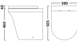
Comfort Height Back To Wall WC Pan BTWC650S
