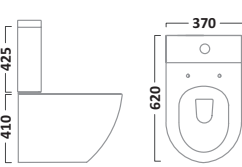
Close Coupled WC Pan P250S Cistern RA453CCC
