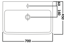
700mm Ceramic Basin I Tap Hole SB357S
