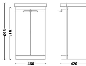
500mm Freestanding Unit Gloss White TE500FW Light Java TE500FLJ Dark Java TE500FDJ Gloss Light Grey TE500FG
