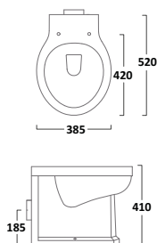
Back To Wall WC Pan BTW850S
