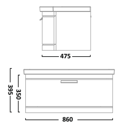
900mm Wall Mounted Unit Gloss White TE900WW Light Java TE900WLJ Dark Java TE900WDJ Gloss Light Grey TE900WG
