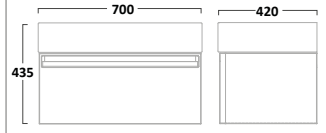
700mm Wall Mounted Unit Gloss White FR70WW Gloss Light Grey FR70WG Gloss Dark Grey FR70WDGG
