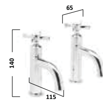
Basin Taps (pair) Chrome TCM70
