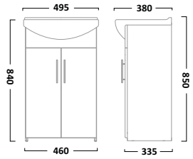
500mm Freestanding Unit Gloss White OPVU50W
