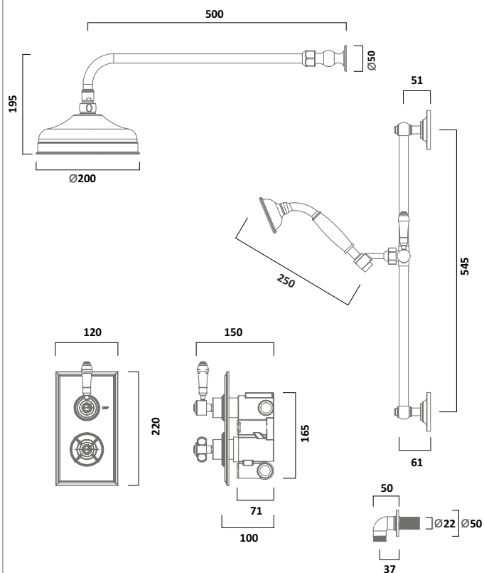
Thermostatic Concealed Dual Function Diverter Shower Valve with Shower Head & Single Function Handset Chrome
