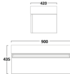
900mm Wall Mounted Unit Gloss White FR90WW Gloss Light Grey FR90WG Gloss Dark Grey FR90WDGG
