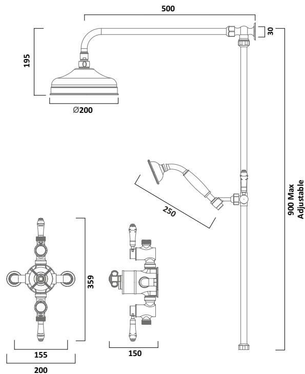
Thermostatic Exposed Dual Function Shower Valve with Shower Head & Handset Chrome
