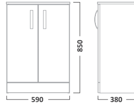
600mm Freestanding Unit Gloss White SWF6W Montana Gloss SWF6MG
