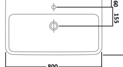
800mm Ceramic Basin I Tap Hole SB358S
