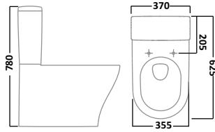
Close Coupled WC Pan P350S Cistern C350S
