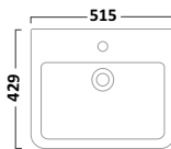
Standard Depth Semi-Countertop Basin I Tap Hole SCSB930S
