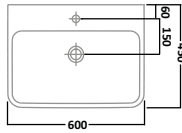
600mm Ceramic Basin I Tap Hole SB356S
