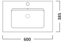
600mm Ceramic Basin Ceramic SW60C
