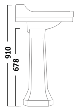
Pedestal Ceramic PE850S
