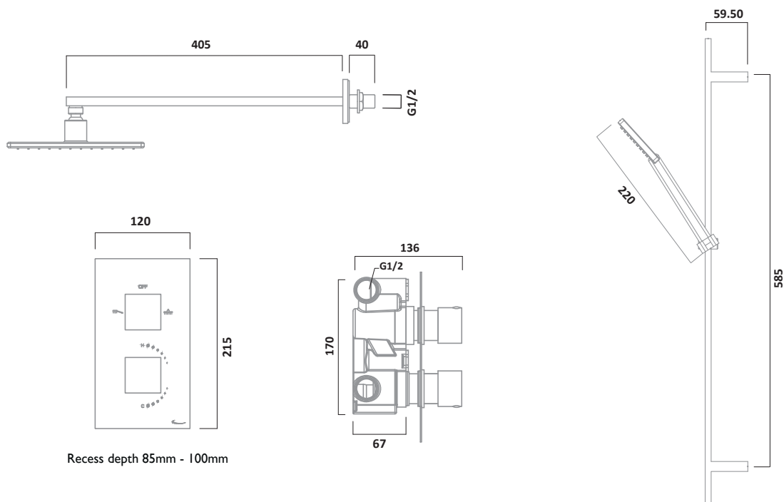
Thermostatic Concealed Dual Function Diverter Valve with 220 x 220mm Square Shower Head & Single Function Shower Handset Chrome SNDI610
