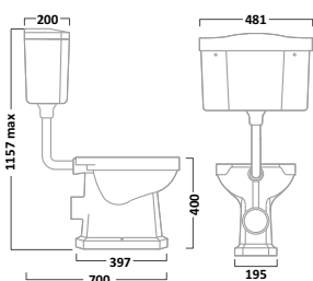
Low Level Cistern inc Fittings & Down Pipe Cistern CL850S Pipe & Fittings LLK850S
