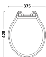
Soft Close Wood WC Seat Solid Oak TS850NOSC
