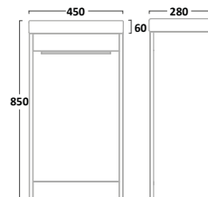
450mm Cloakroom Unit Gloss White SQ450FW Gloss Light Grey SQ450FG Gloss Clay SQ450FC
