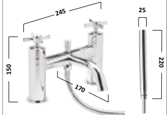
Bath Shower Mixer & Handset Chrome TCM42
