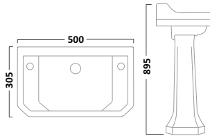
500mm Cloakroom Basin I Tap Hole DB850CLS
