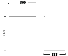
Back To Wall WC Unit Gloss White OPBTW50W
