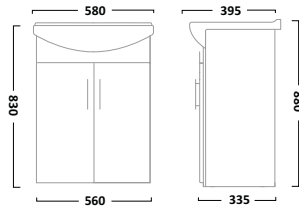
600mm Freestanding Unit Gloss White OPVU60W
