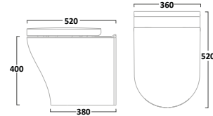
Back To Wall WC Pan BTW350S
