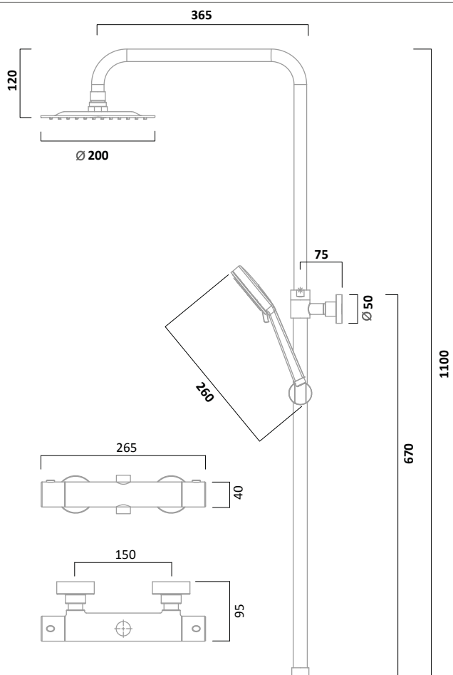
Thermostatic Diverter Bar Valve with 200mm Round Stainless Steel Shower Head and Multi Function Shower Handset Chrome SQT1509
