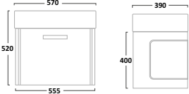
570mm Wall Mounted Unit Gloss White Q600W Graphite Q600G
