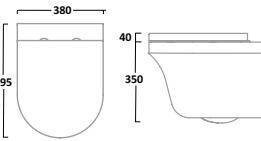
Comfort Height Wall Hung WC Pan WH650S
