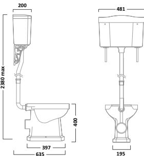
High Level Cistern, Chrome Down Pipe & Bracket Kit Cistern CH850S Pipe & Chain HLK850S
