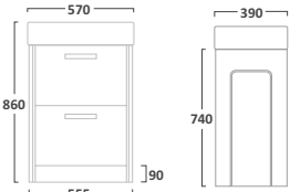
570mm Freestanding Unit Gloss White Q6FW Graphite Q6FG
