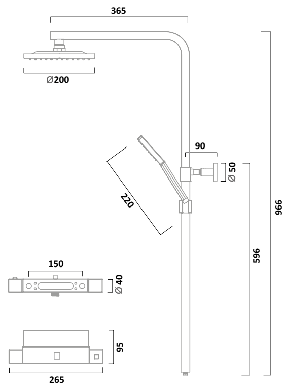
Dual Function Bar Valve with Shower Head & Handset Chrome SZNI508
