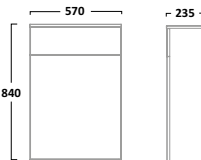
Back To Wall WC Unit Gloss White DC12009
