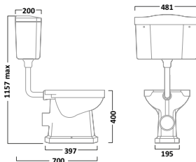
Low Level Cistern inc Fittings & Down Pipe Cistern CL850S Pipe & Fittings LLK850S
