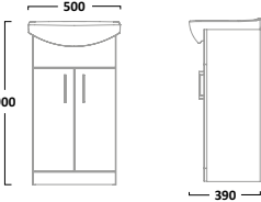
500mm Freestanding Unit Gloss White DC1200F
