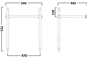
Washstand Chrome DC140Z4
