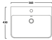
Semi-Countertop Basin 1 Tap Hole DC1400Z
