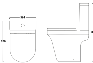
Comfort Height Open Back Close Coupled WC inc Floor Fittings Pan PC650S Cistern C650S
