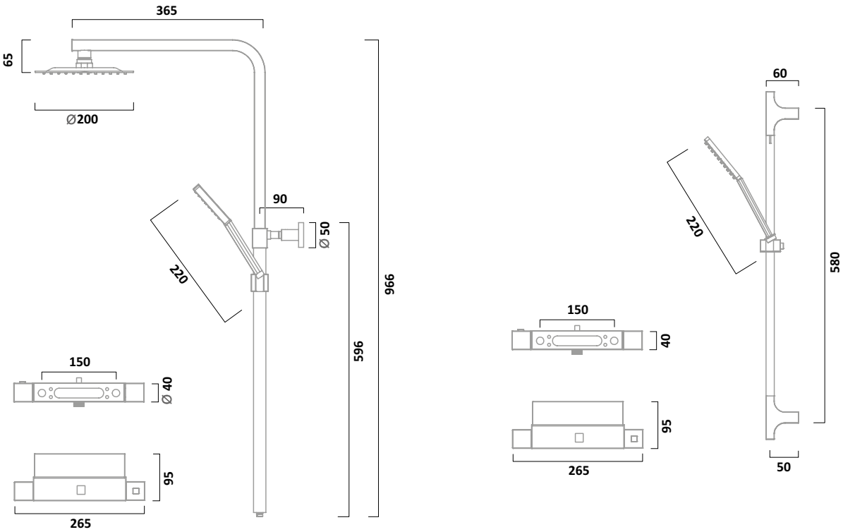
Thermostatic Dual Function Bar Valve and Accessory Shelf with Shower Head & Handset Chrome SND2008
