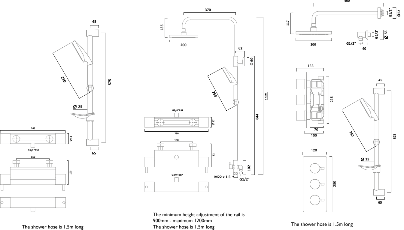
The shower hose is 1.5m long
