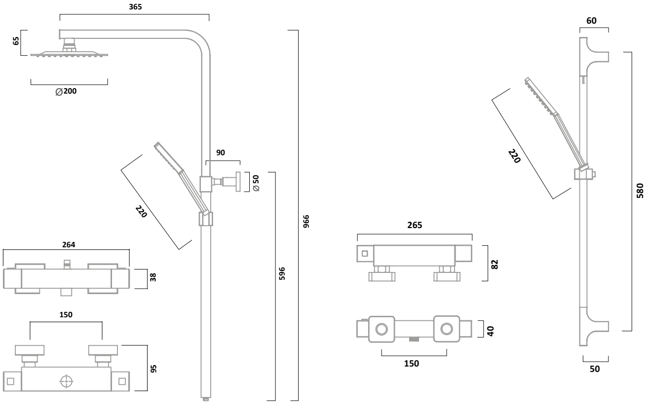
Cool Touch Thermostatic Dual Function Bar Valve with Shower Head & Handset Chrome SND2208
