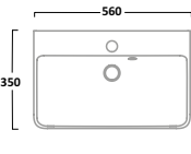
Slim Depth Semi-Countertop Basin 1 Tap Hole DC14003
