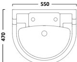
550mm Round Ceramic Basin 1 Tap Hole SB855S 2 Tap Holes DB855S
