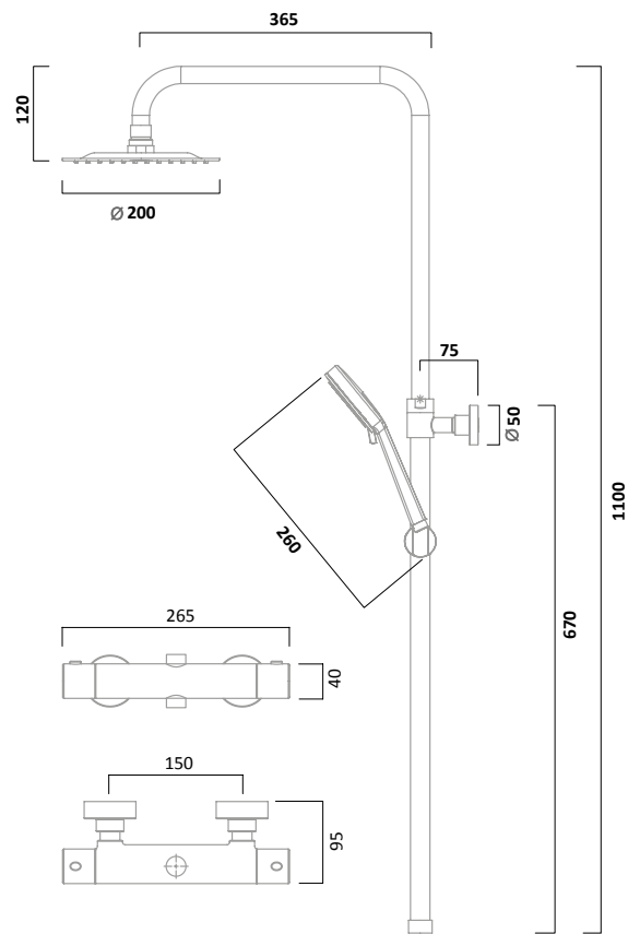
Cool Touch Thermostatic Dual Function Bar Valve with Shower Head & Handset Chrome SQT2209
