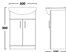
600mm Freestanding Unit Gloss White DC12008
