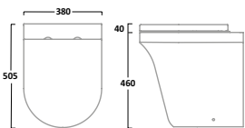
Comfort Height Back To Wall WC Pan BTWC650S
