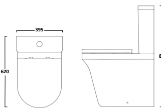
Comfort Height Fully Enclosed Close Coupled WC Pan PCF650S Cistern C650S
