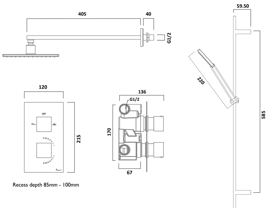
Thermostatic Concealed Dual Function Valve with Shower Head & Handset Chrome SND1610
