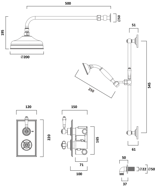
Thermostatic Concealed Dual Function Shower Valve with Shower Head & Handset Chrome SVA1615
